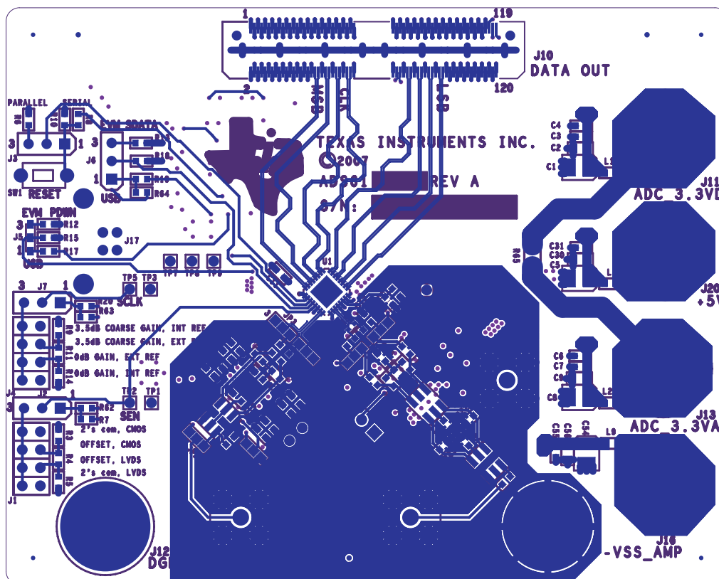
Figure 2. Top Silkscreen
