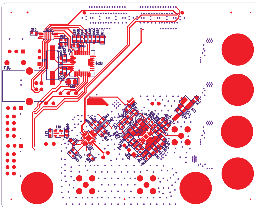
Figure 6. Bottom Side
